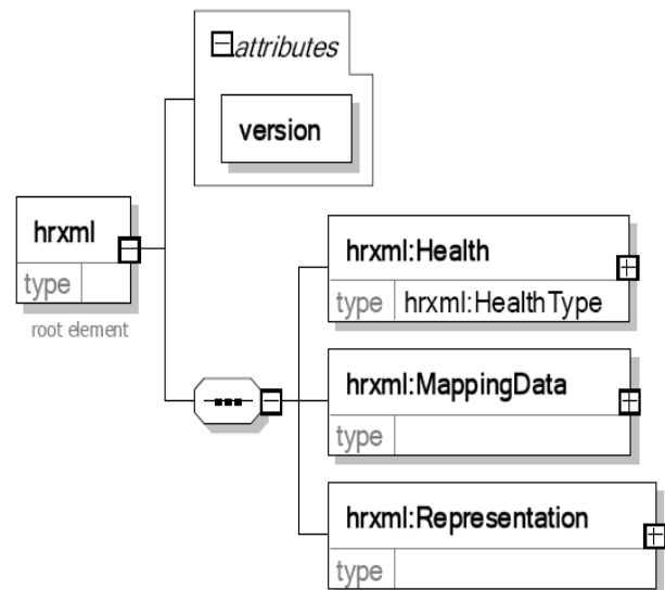
Figure 1. HRXML schema
